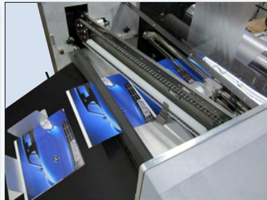
Diagonal Cutter
